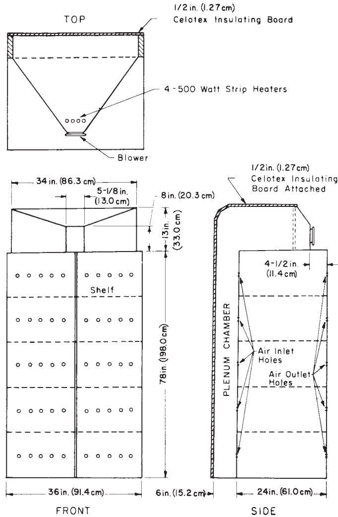
FIG. 2 Air-Drying Oven
