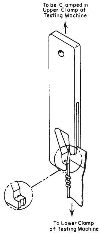
FIG. 9 Fixture for Separable Pin Pull-Off Test
