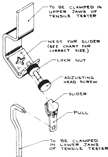
FIG. 20 Fixture for Angular Pull, Pull-Off Test
