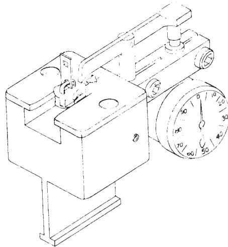
FIG. 15 Fixture for Slider Deflection Test (Pull)
