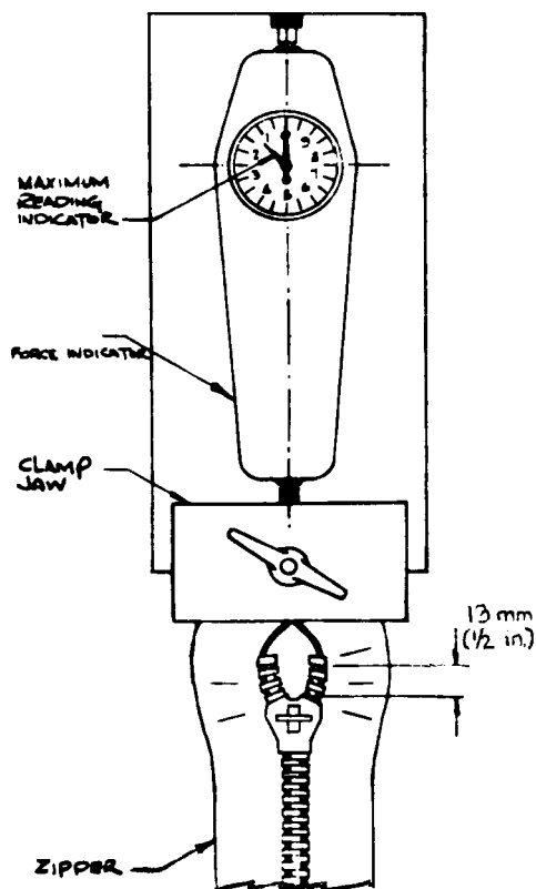
FIG. 3 Chain Opening
