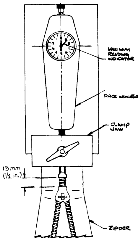
FIG. 4 Chain Closing
