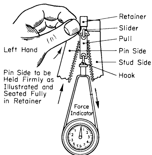
FIG. 5 Pin Fully Seated in Retainer
