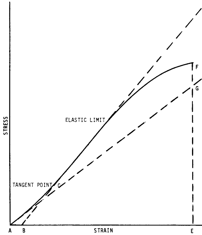
FIG. X1.1 Material with Hookean Region
