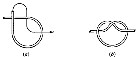
FIG. A1.2 Type "U" Knot
