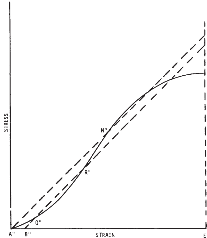
FIG. X2.1 Construction for Chord Modulus
