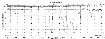
FIG. 22 Infrared Absorption Spectrum of a Typical Triacetate Fiber
