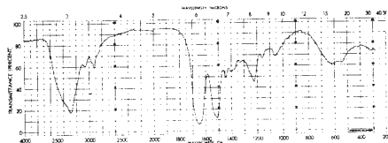
FIG. 20 Infrared Absorption Spectrum of a Typical Silk Fiber
