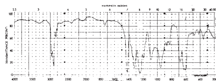
FIG. 24 Infrared Absorption Spectra of Typical Vinyon Fibers
