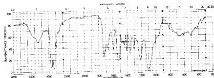
FIG. 21 Infrared Absorption Spectrum of a Typical Spandex Fiber
