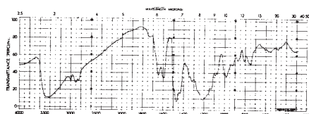
Kynol® FIG. 12 Infrared Absorption Spectrum of a Typical Novoloid Fiber
