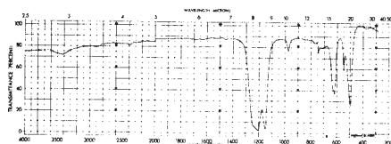
Teflon® FIG. 9 Infrared Absorption Spectrum of a Typical Fluorocarbon Fiber
