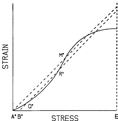
FIG. X2.1 Example of Construction for Chord Modulus
