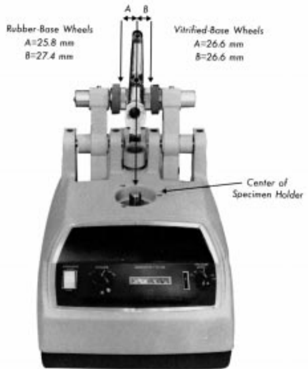
FIG. 2 Position of Abrasive Wheels on Rotary Platform Double Head Abraser
