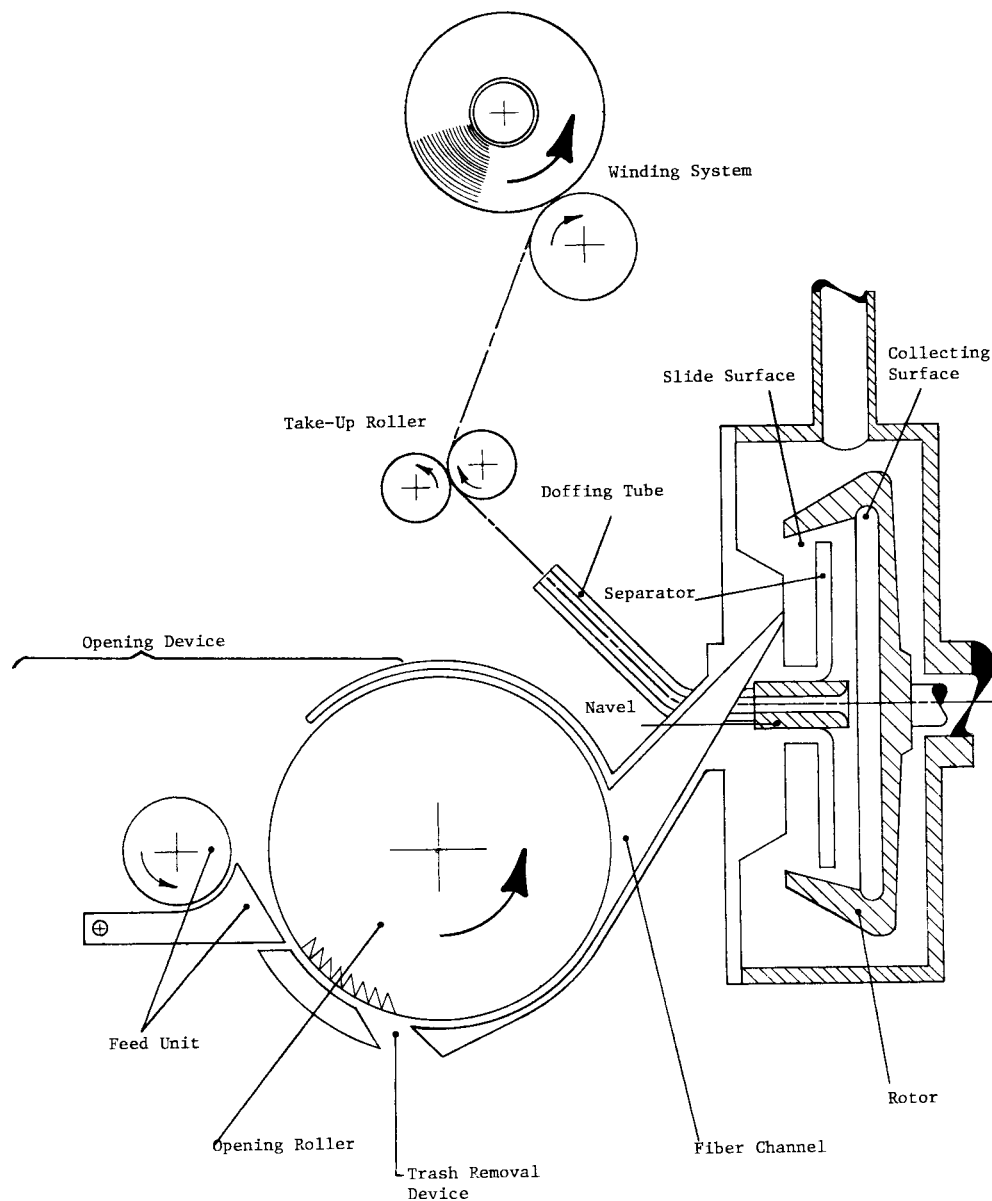
FIG. 1 Schematic Diagram of Open-End Spinning Machine
