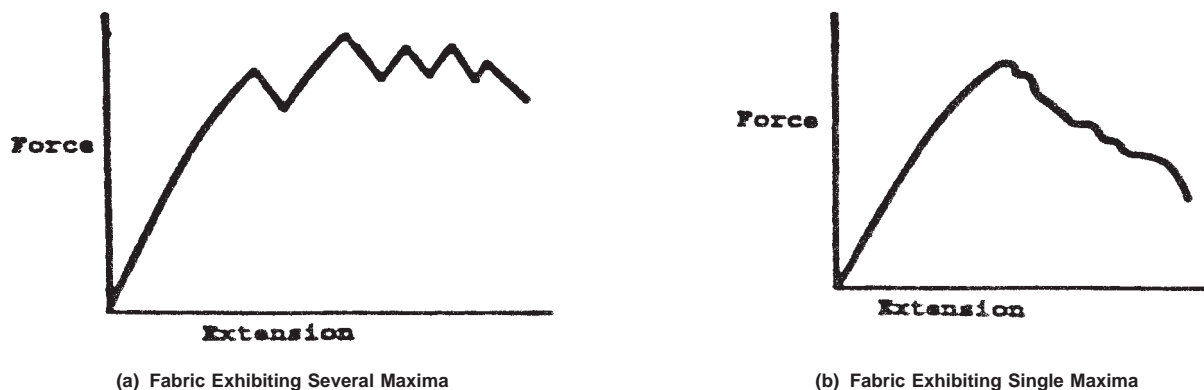
FIG. 3 Typical Trapezoid Tearing Force-Extension Curves for Individual Specimens
