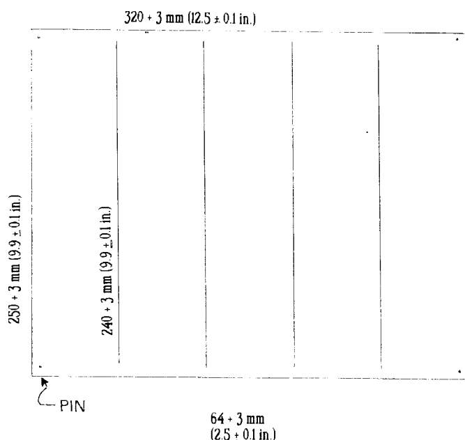
FIG. A1.1 Template for 250 by 320-mm Specimen
