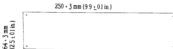
FIG. A1.2 Template for 64 by 250-mm Specimen
