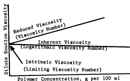
FIG. X1.1 Example of Plot to Determine Intrinsic Viscosity.
