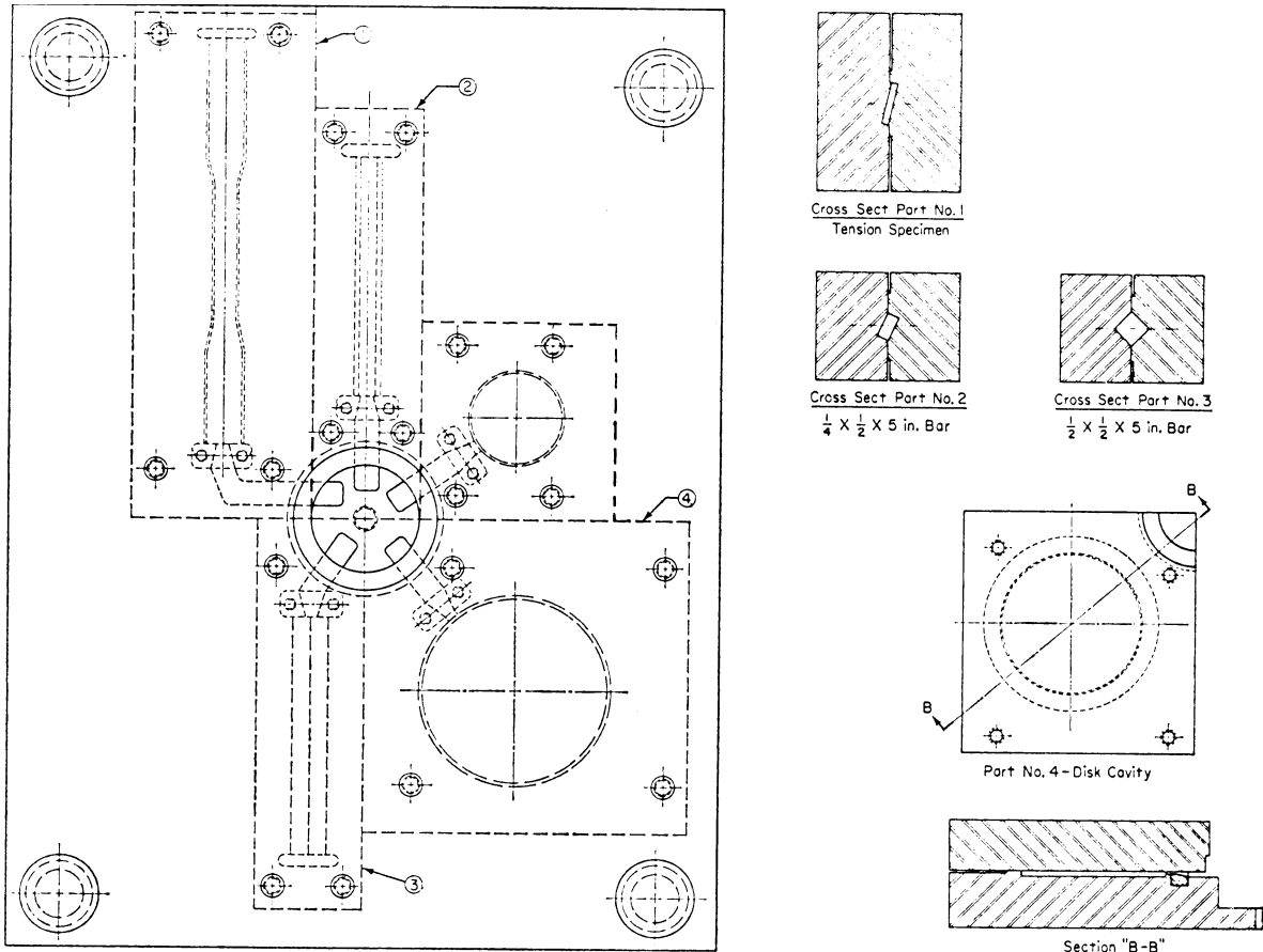
FIG. 1 Five-Cavity Transfer Mold for Thermosetting Plastic Test Specimens (Steam Cores Not Shown)
