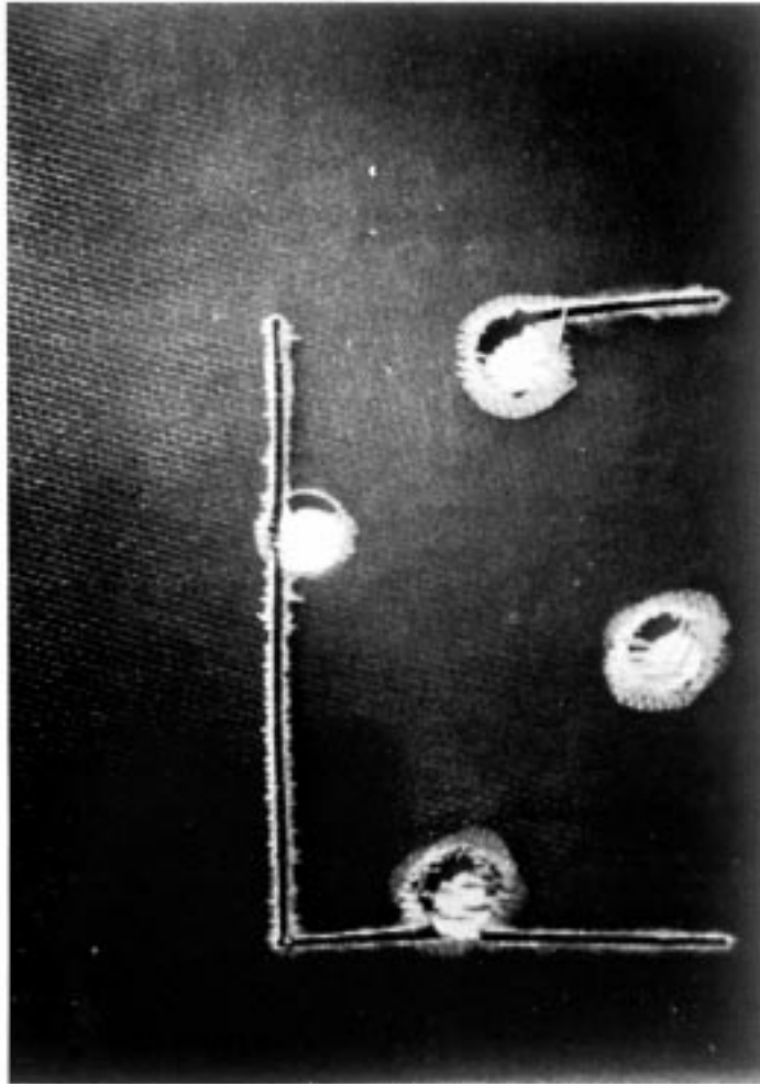
FIG. 3 Delamination by Improper Machining
