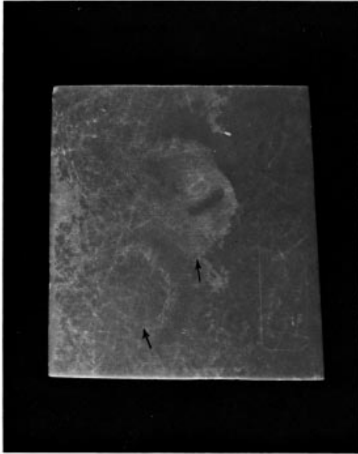
FIG. 10 Fish Eye
