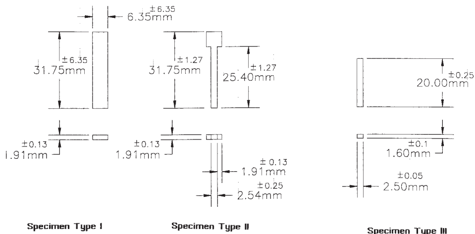
FIG. 6 Specimen Geometry
