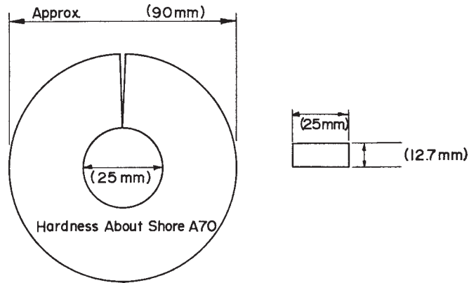
FIG. X1.2 Rubber Bumper
