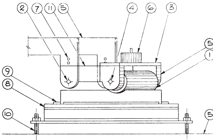
FIG. X2.2 Roller Shear Machine—Side View
