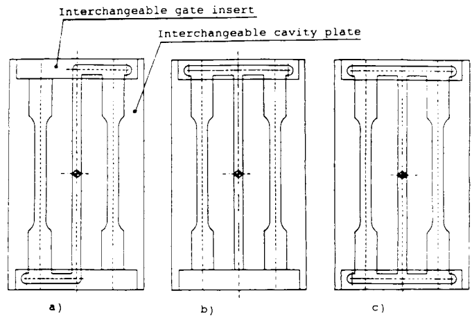
FIG. A1.2 Cavity Layout for Large Tensile Specimens
