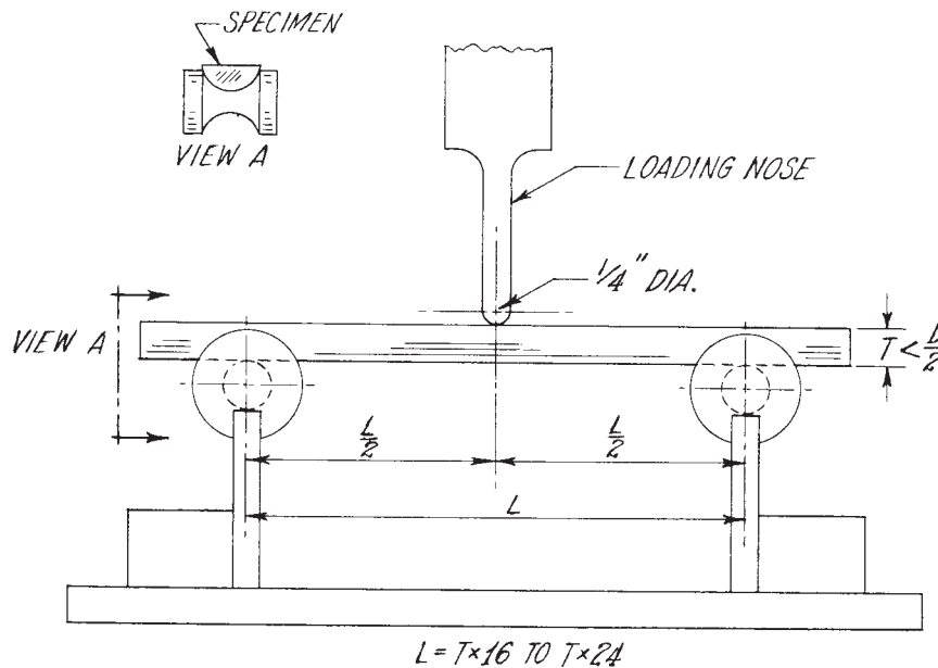
FIG. 3 Schematic of Flexural Test
