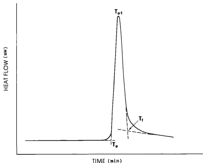
FIG. 2 Cooling Curve
