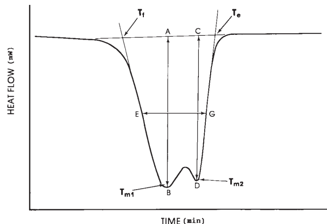
FIG. 1 Heating Curve
