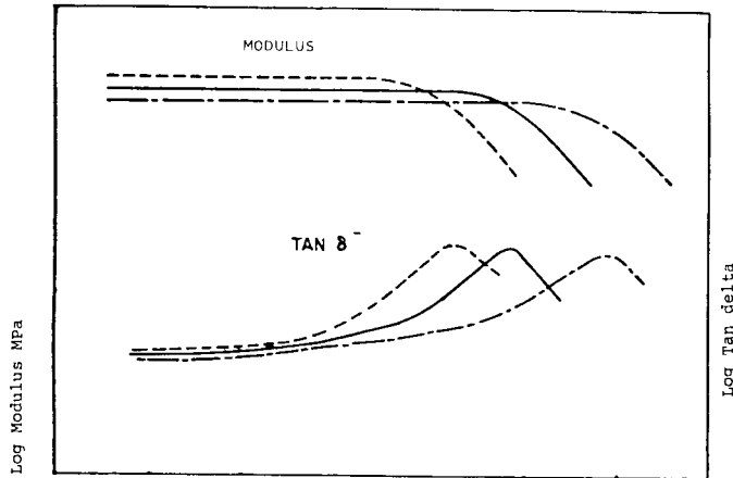
TEMPERATURE FIG. 1 Dynamic Mechanical Properties in Tension (at Different Frequencies)
