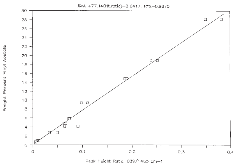
FIG. 2 Vinyl Acetate Correlation Curve (609 \text{cm}^{-1} /1465 \text{cm}^{-1} Height Ratio) Prepared Using Procedure B
