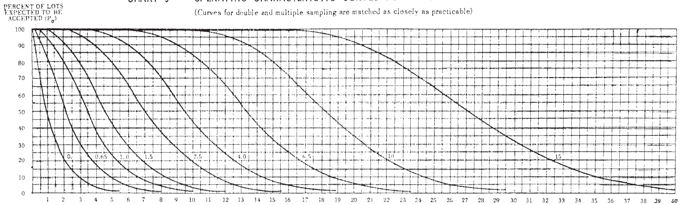
CHART J - OPERATING CHARACTERISTIC CURVES FOR SINGLE SAMPLING PLANS
