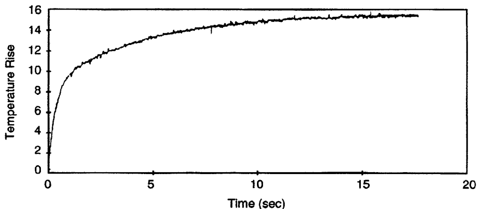
FIG. 9 Typical Sensor Temperature Rise Curve with Time Scale and Baseline Correction
