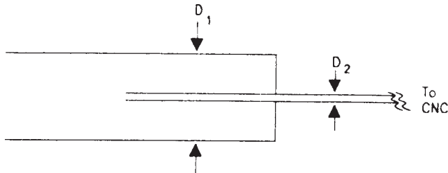
FIG. 2 Isokinetic Sampler Calculation
