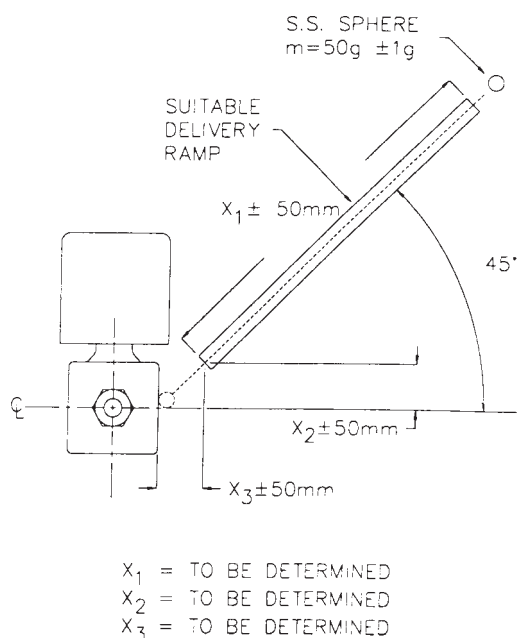
FIG. 4 Mechanical Shock Device
