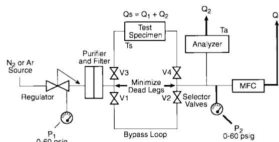
FIG. 1 Test Schematic
