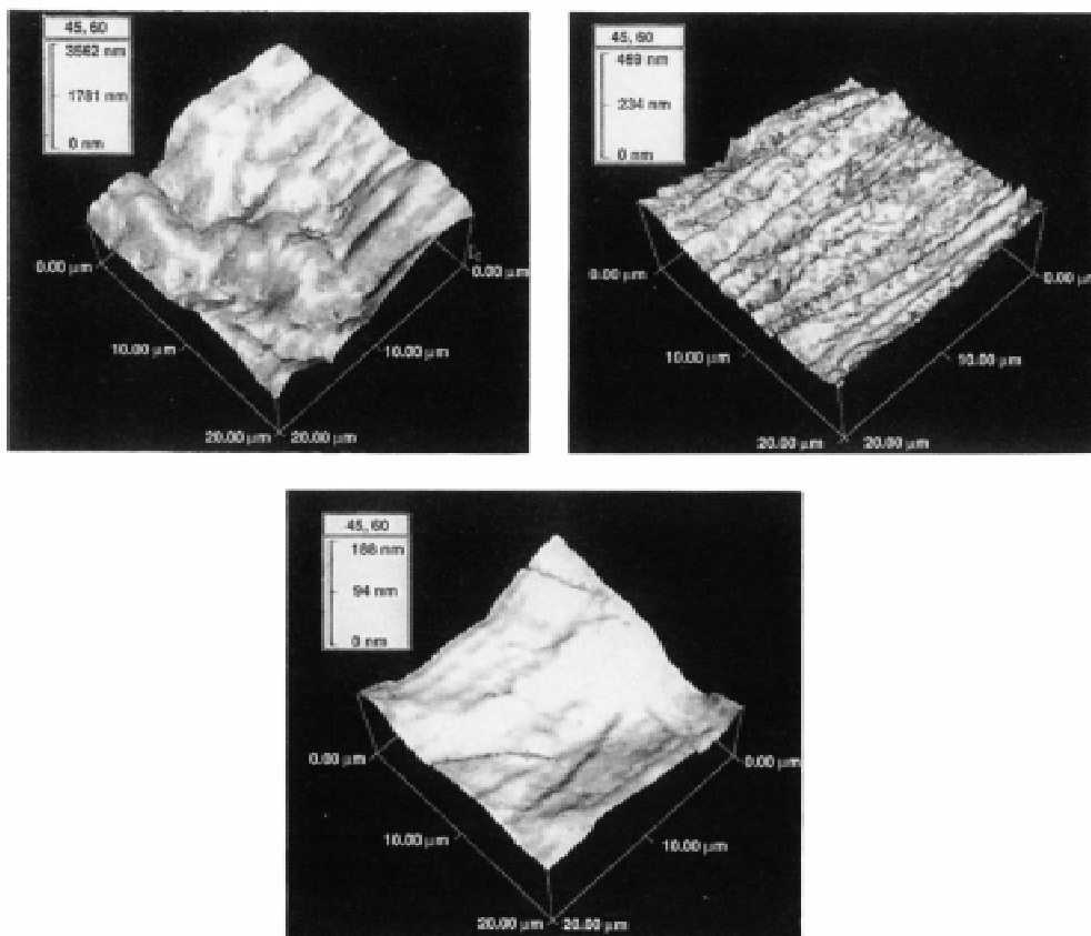
FIG. 9 Stainless Steel Surfaces Used for SA Index, Z_{\max} , and Z_{\text{rms}} Data Given in Table 1
