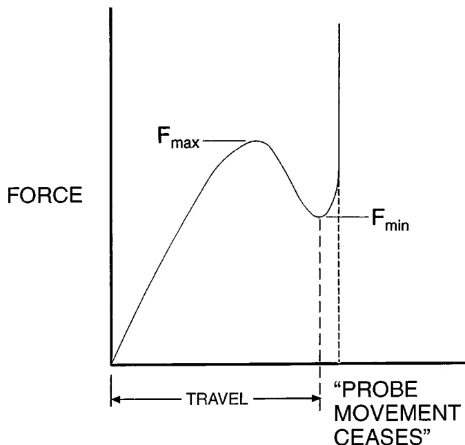
FIG. 1 Typical Tactile Force—Travel Curve
