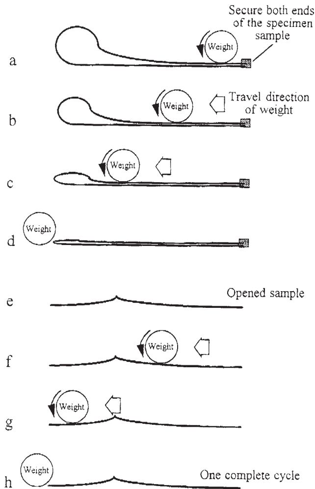
FIG. 2 Crease Cycle
