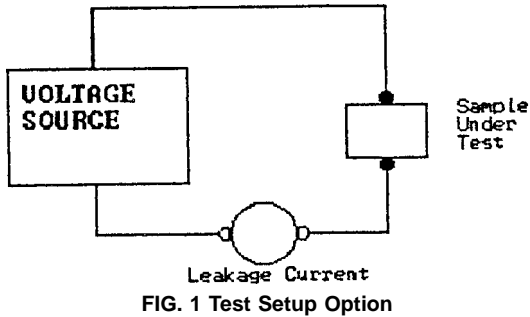
FIG. 1 Test Setup Option
