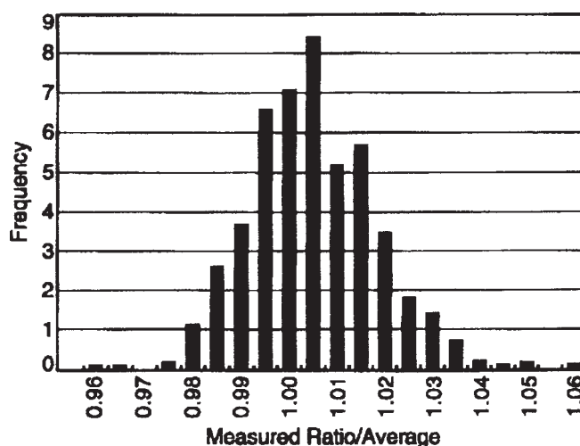
NOTE 1—The distribution demonstrates the stringent reproducibility capable of a controlled RBS instrument.
