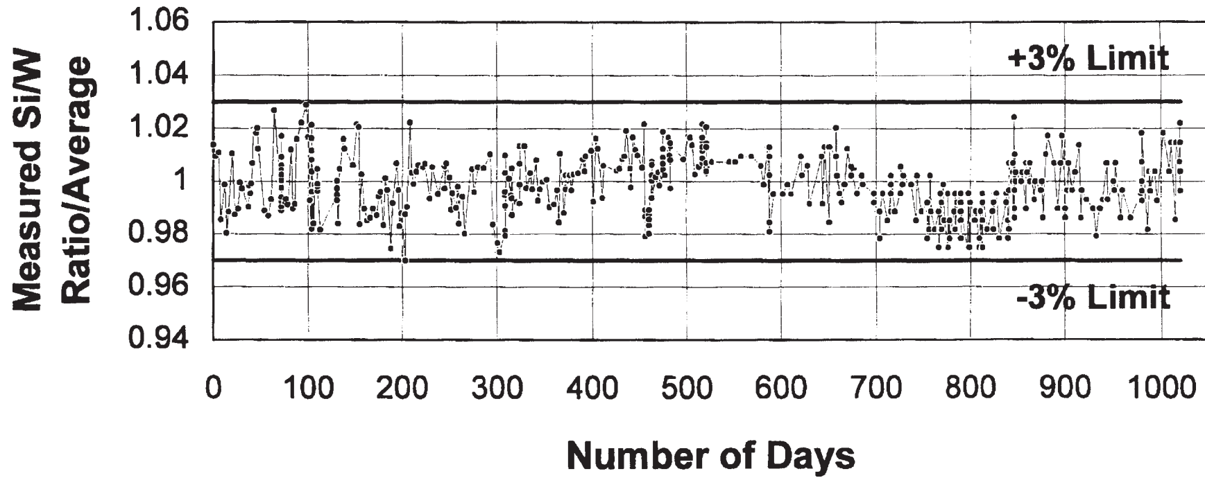
FIG. 4 Running Plot of Measured Silicon/Tungsten Ratios Obtained in an SPC Program.
