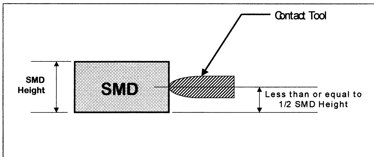
FIG. 1 SMD Contact
