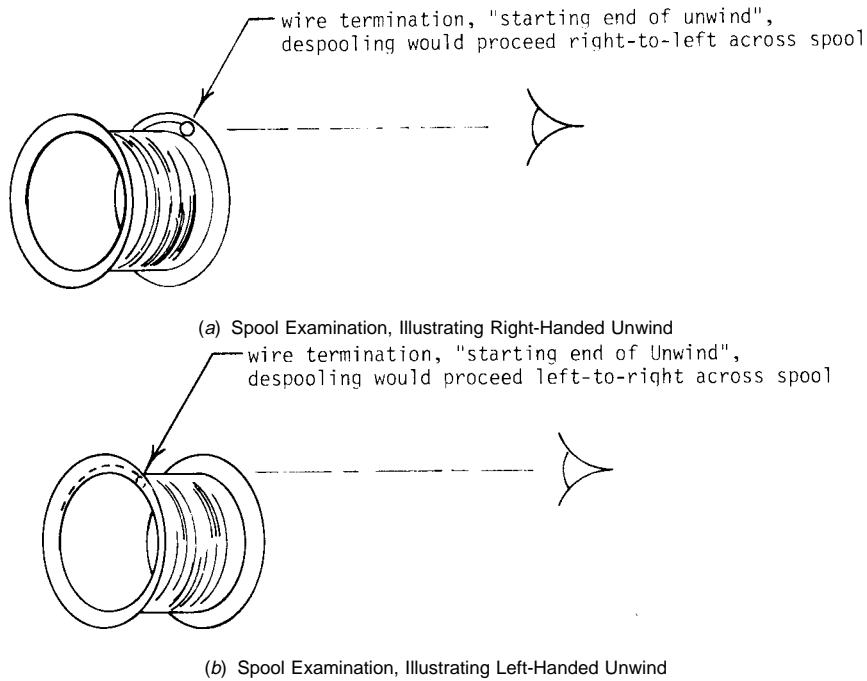
FIG. 11 Test Arrangement, Determination of Handedness of Wire Unwind
