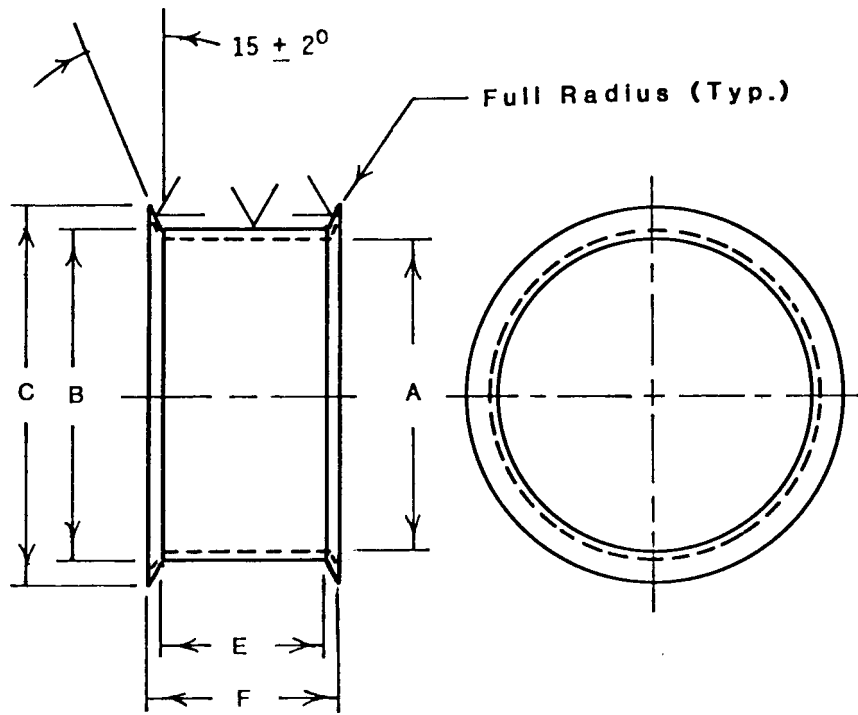
FIG. 4 Large Phenolic Plastic Spool
