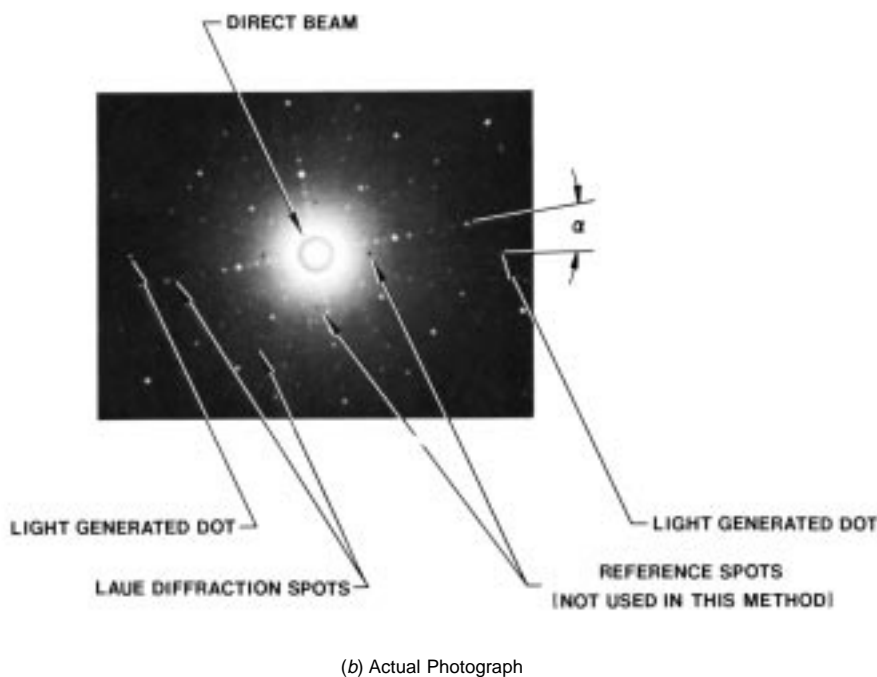
FIG. 6 Laue Pattern
