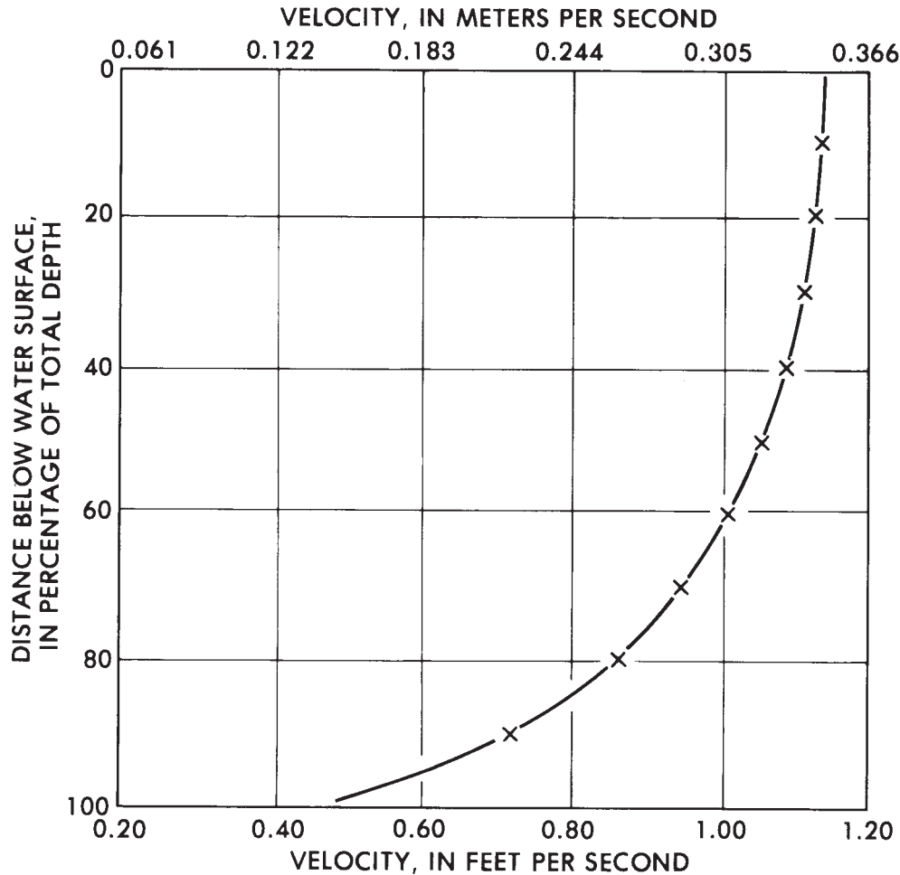
FIG. 1 Typical Open-Channel Vertical-Velocity Curve (Modified from Buchanan and Somers) 7
