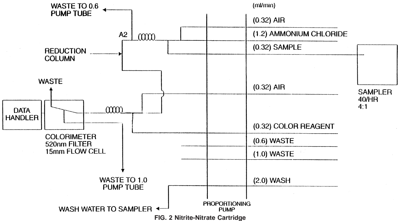
FIG. 2 Nitrite-Nitrate Cartridge
