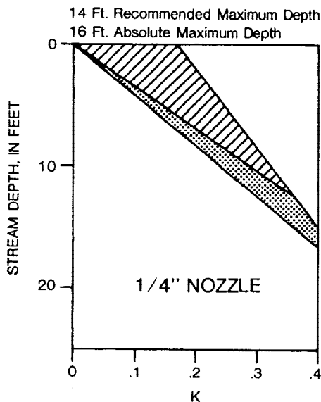
FIG. 9 (18) Transit Rates for Depth-Integrating Sampler Type US D-74 with Quart Sample Container
