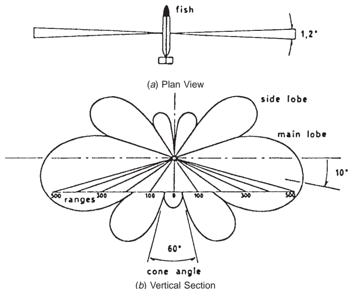
FIG. 13 Towfish Tethered to Survey Vessel Producing Lobe-figure of Side Scan Sonar Beam (14)
