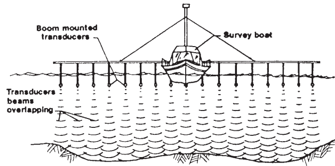
FIG. 11 Channel Sweep System
