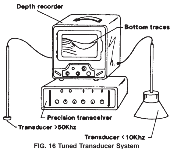
FIG. 16 Tuned Transducer System
