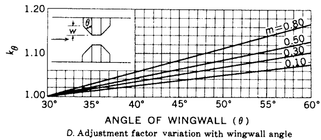
FIG. 15 Coefficients for Type 4 Opening, Embankment Slope 2 to 1, Vertical Abutments With Wingwalls
