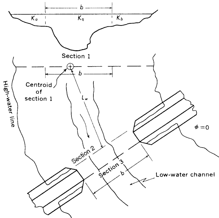
B. Condition of channel curvature
