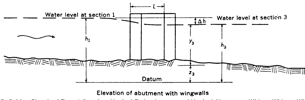
FIG. 3 Definition Sketch of Type 1 Opening, Vertical Embankments and Vertical Abutments With or Without Wingwalls
