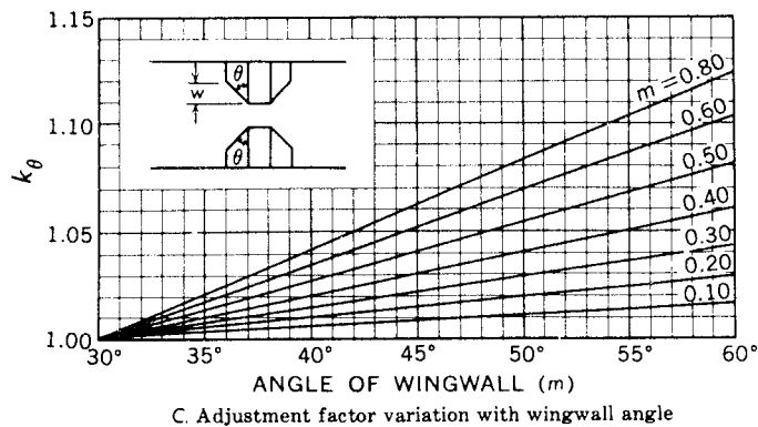
FIG. 14 Coefficients for Type 4 Opening, Embankment Slope 1 to 1, Vertical Abutments With Wingwalls
