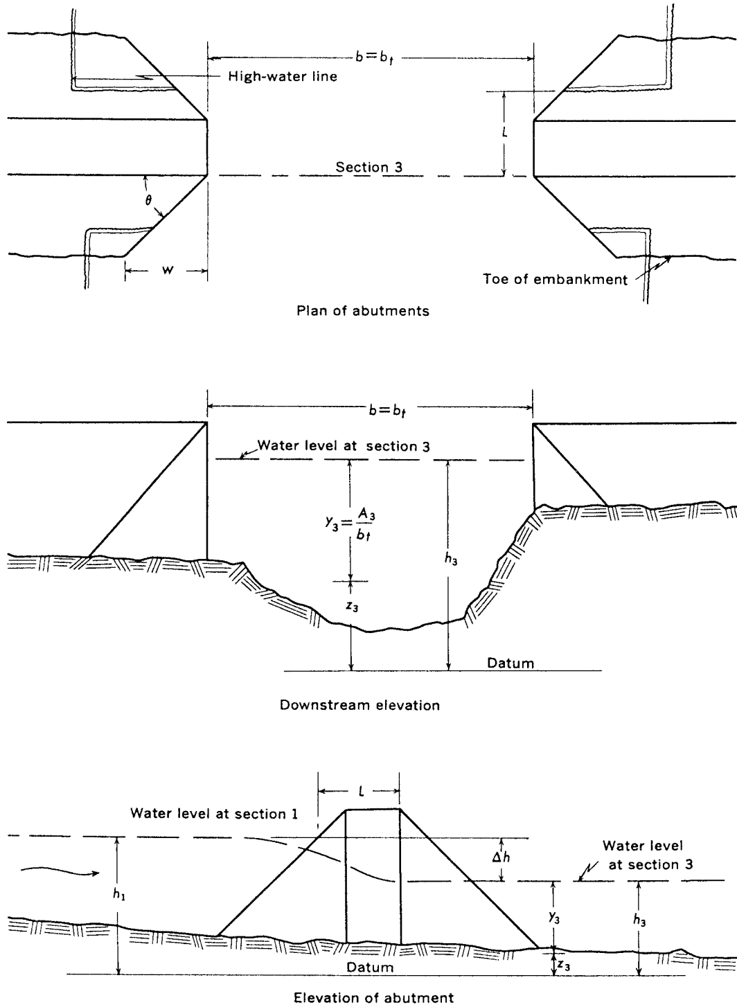
FIG. 6 Definition Sketch of a Type 4 Opening, Sloping Embankments and Vertical Abutments With Wingwalls
