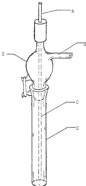
A Inlet, from sample air outlet B Outlet, to standard scrubber C Tube, extends into scrubber solution D Body, glass with 1\frac{1}{2} standard-taper joint, total length 125 mm, used with up to 12-mL scrubber solution E Adaptor, glass
