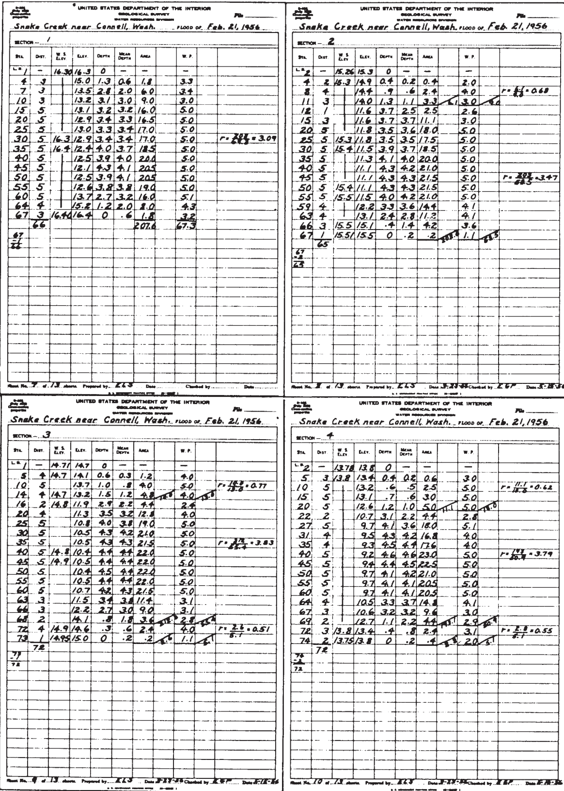
FIG. 7 Sample Slope-Area Computation, Cross-Section Properties
