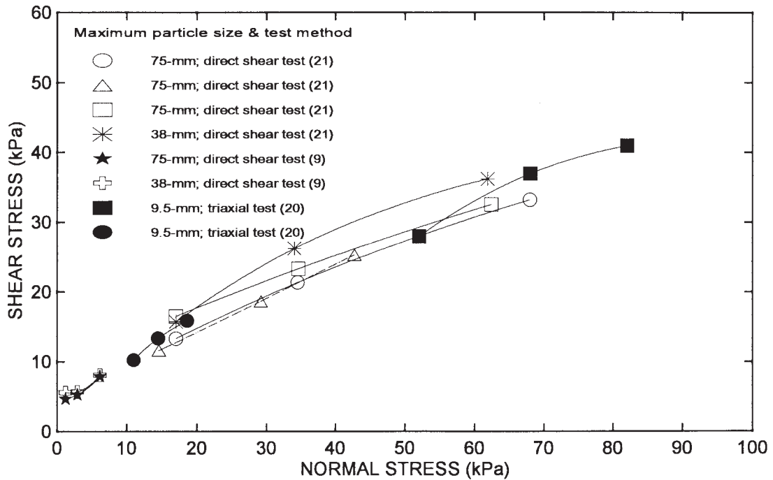
FIG. X1.3 Comparison of Failure Envelopes of Tire Shreds at Low Stress Levels
