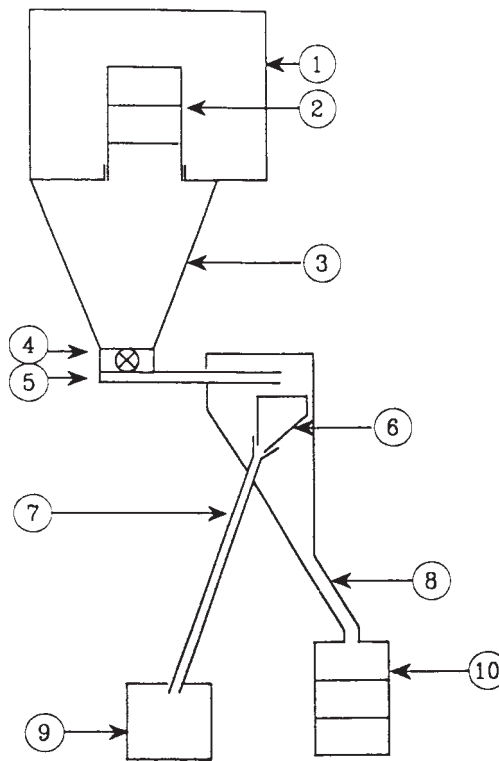
FIG. 5 Schematic Diagram of Vezin Secondary Sampler
