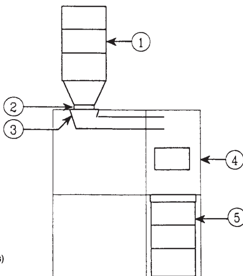
FIG. 4 Schematic Diagram of Reciprocating-Cutter Secondary Sampler
