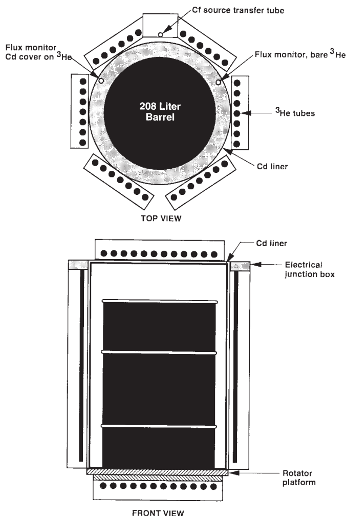
SHUFFLER DETECTOR BANK DIAGRAM
