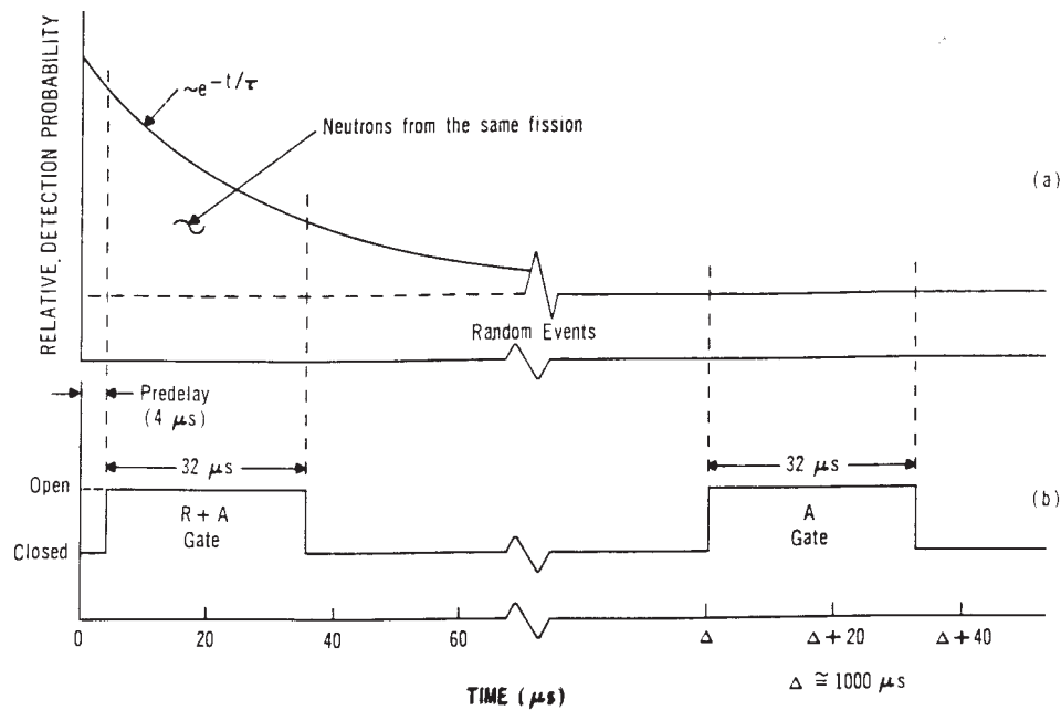
a) Simplified relative neutron detection probability distribution.
