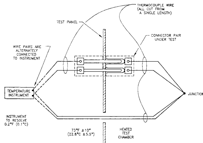
FIG. 3 Miniature Thermocouple Connector Test Circuit Diagram
