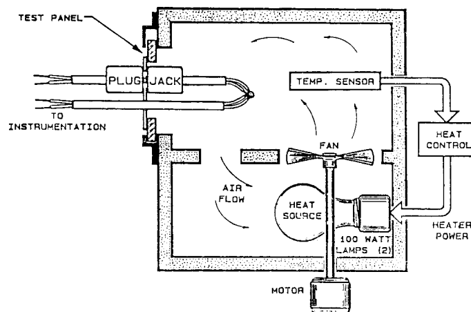
FIG. 2 General Arrangement for Thermal Gradient Test
