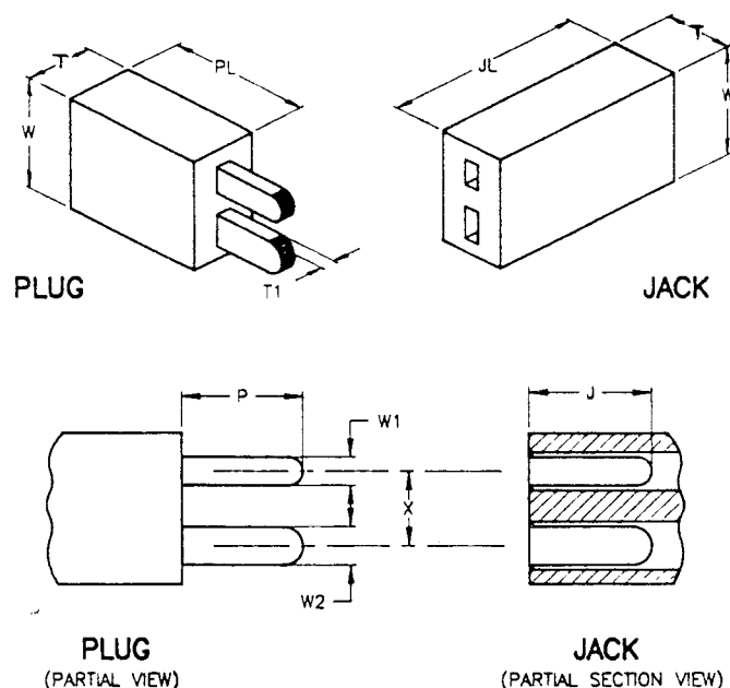
FIG. 1 Miniature Thermocouple Connector Dimensions (see Table 1)
