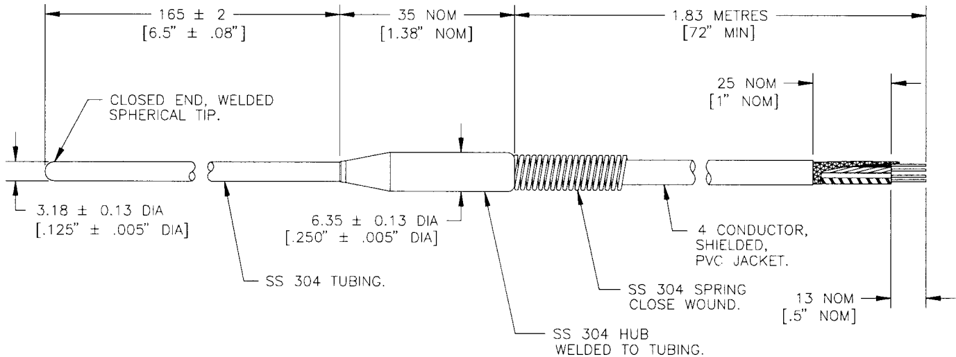
NOTE 1—Metric (English) All dimensions in millimetres unless otherwise indicated. FIG. 4 General Purpose Four-Wire Sensor in Stainless Steel Housing
