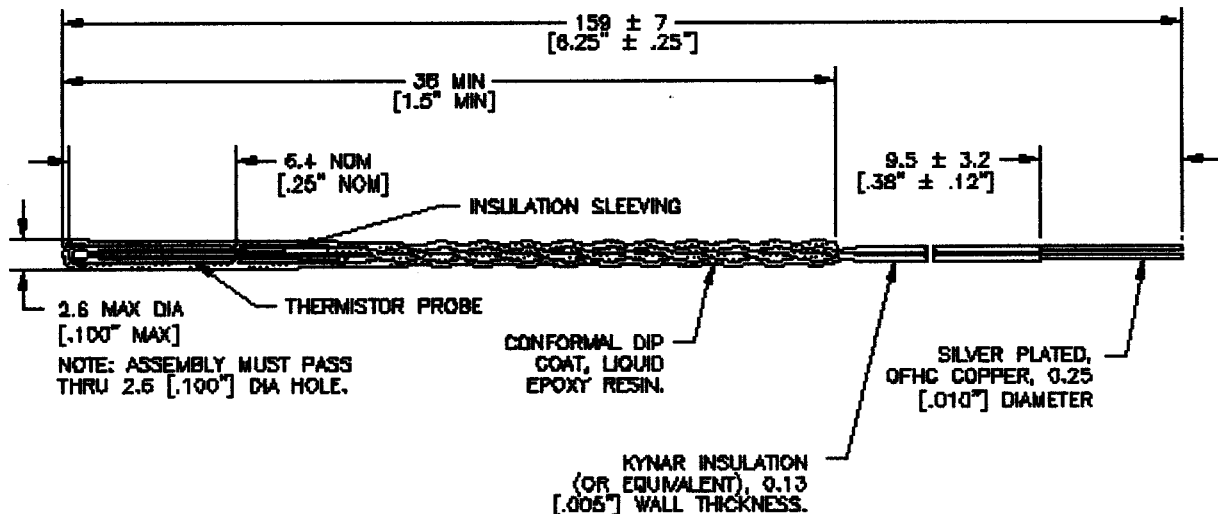
FIG. 3 Epoxy Coated Glass Probe
