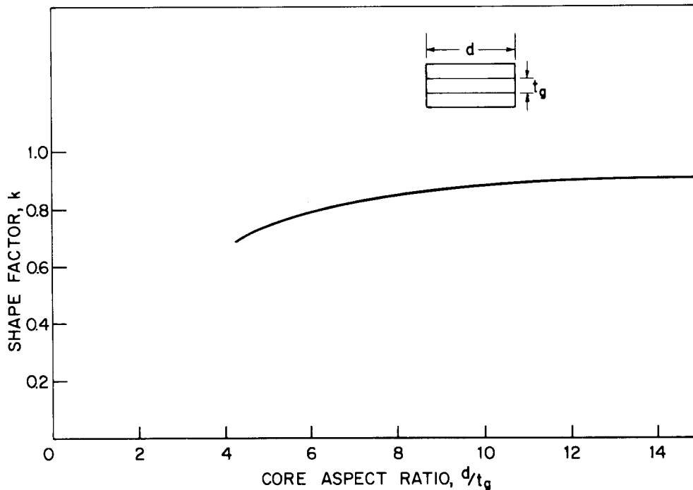
FIG. 3 Shape Factor
