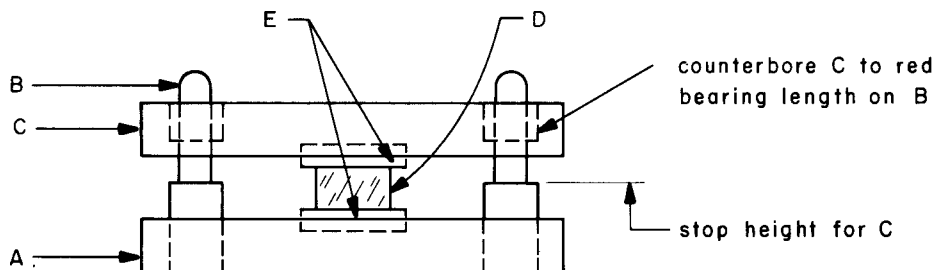
FIG. A2.1 Furnace Sealing Fixture
