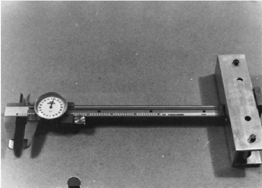
FIG. 2 Measurement of Test Bar Deflection with Depth Gauge of Vernier Caliper
