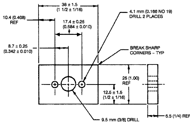
FIG. 4 Test Fixture Center Loading Bar
