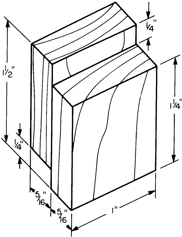
FIG. 2 Modified Block Shear Specimen
