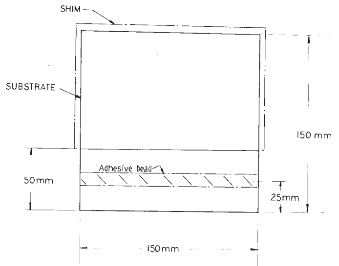
FIG. 4 Placement of Adhesive Bead
