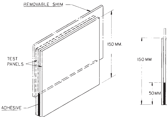
FIG. 5 Test Specimen
